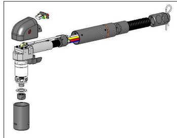
Adapter with long screwing head
