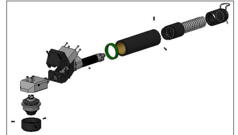
Adapter with extra-short screwing head
